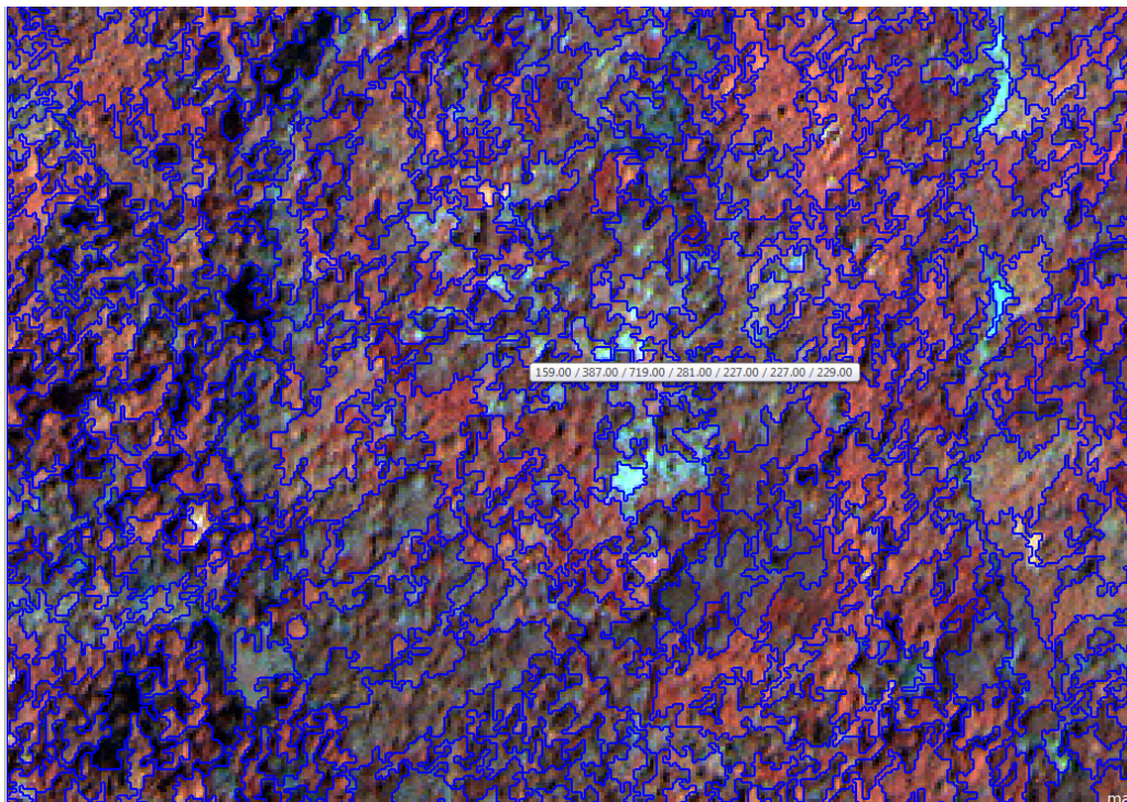
Figure 17. The 6 layer mix false color composite.
